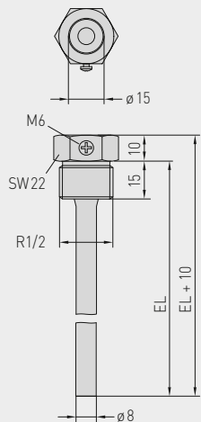
Dimensional drawing TH08- ms /xx
